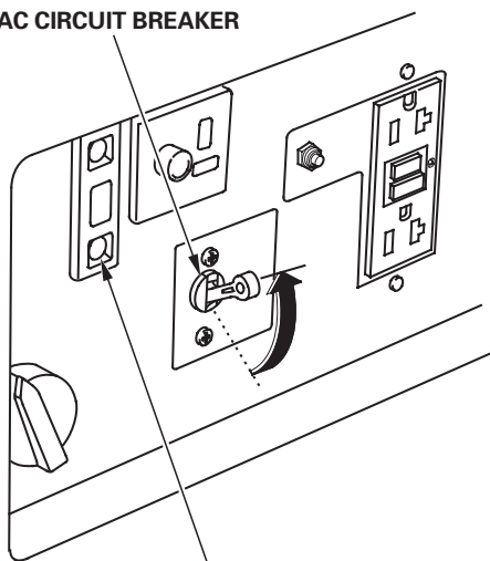
OUTPUT INDICATOR LIGHT (GREEN)
