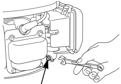
DRAIN BOLT
