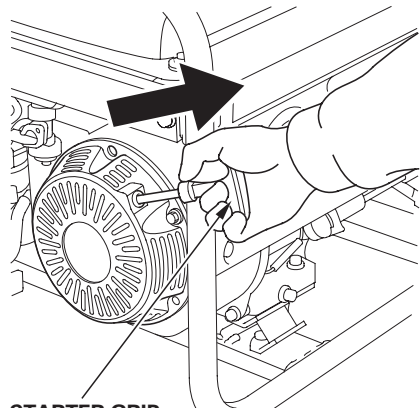
STARTER GRIP
