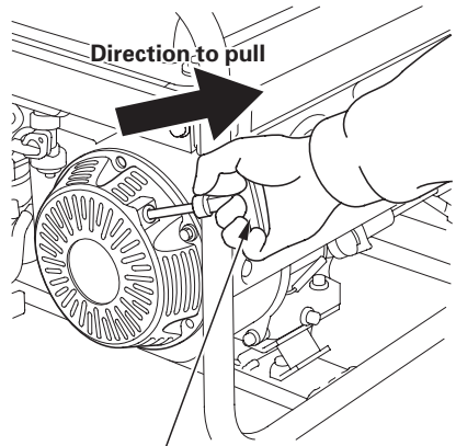
STARTER GRIP
