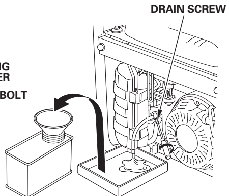
CALIFORNIA TYPE
