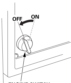
ENGINE SWITCH
