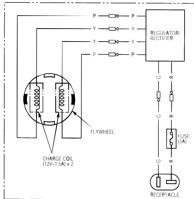
CHARGE RECEPTACLE KIT (OPTIONAL)
