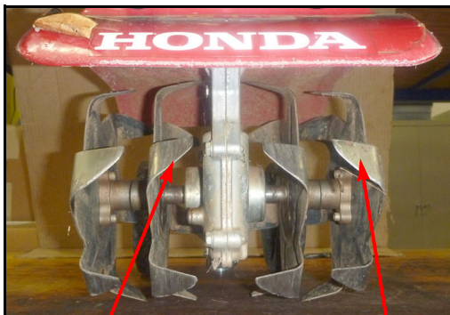
CORRECT INSTALLATION (Viewed from the front)
