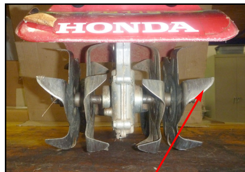
INCORRECT INSTALLATION (Viewed from the front)
