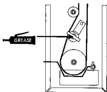
772QAAAA.CDR Drive belt tension arm pivot (gear transmission model only)
