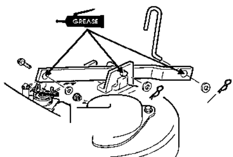
771DACAB.CDR Rear mower deck pivot points
