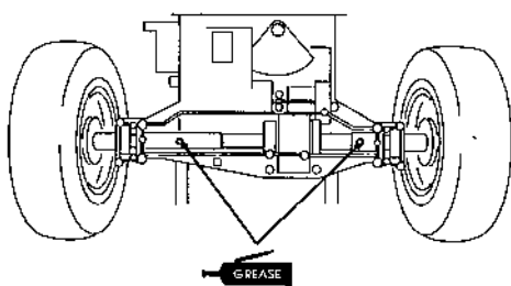
772JACAA.CDR Rear axle shaft grease fittings (gear transmission model only)
