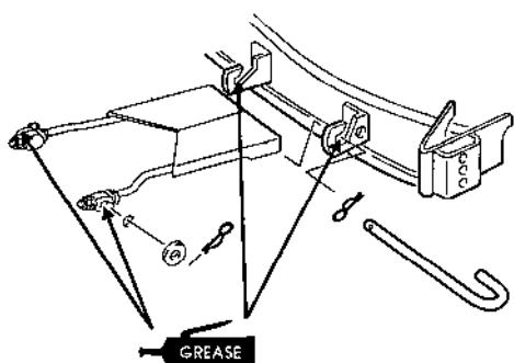
771DADAD.CDR Front mower deck pivot points
