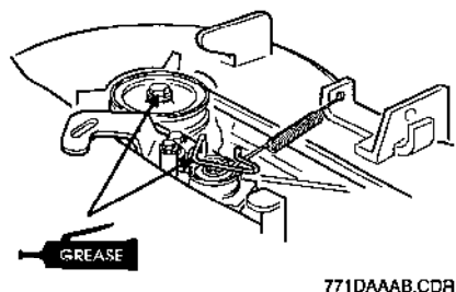
771DAAA.B.CDR Blade belt tension arm pivot
