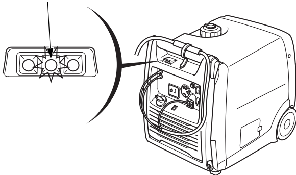
OVERLOAD INDICATOR
