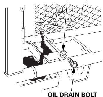
SEALING WASHER (Replace)
