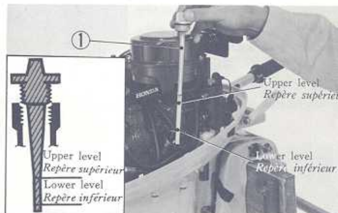
① Oil dipstick
