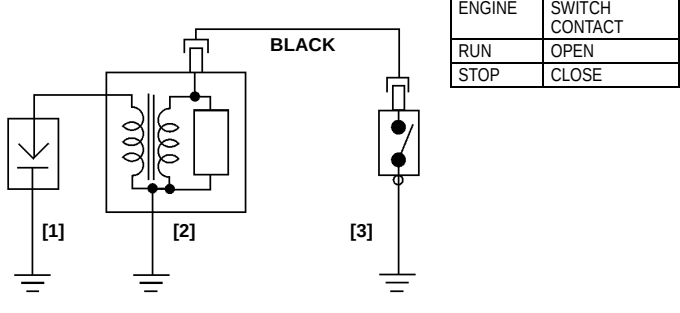
ELECTRIC STARTER (with flywheel brake)
